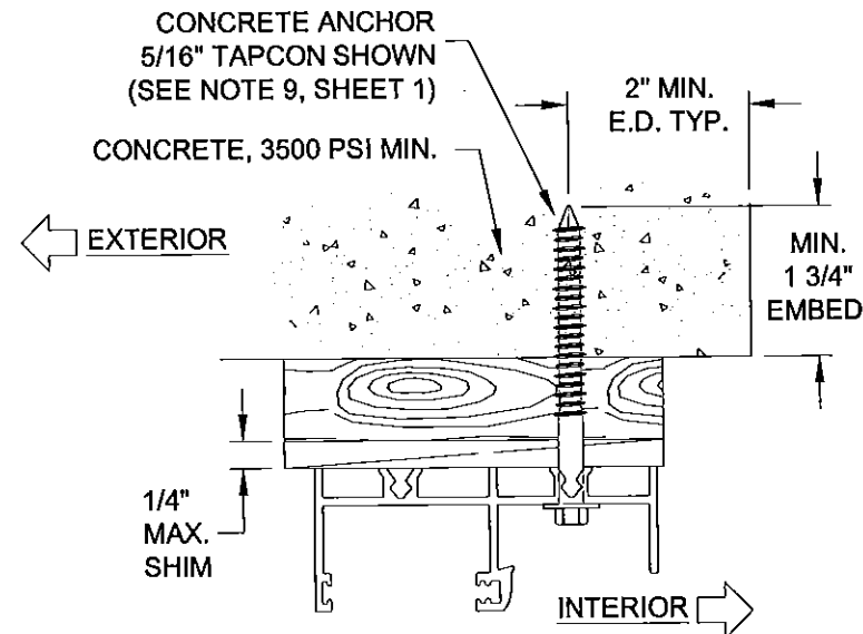
DETAIL B
